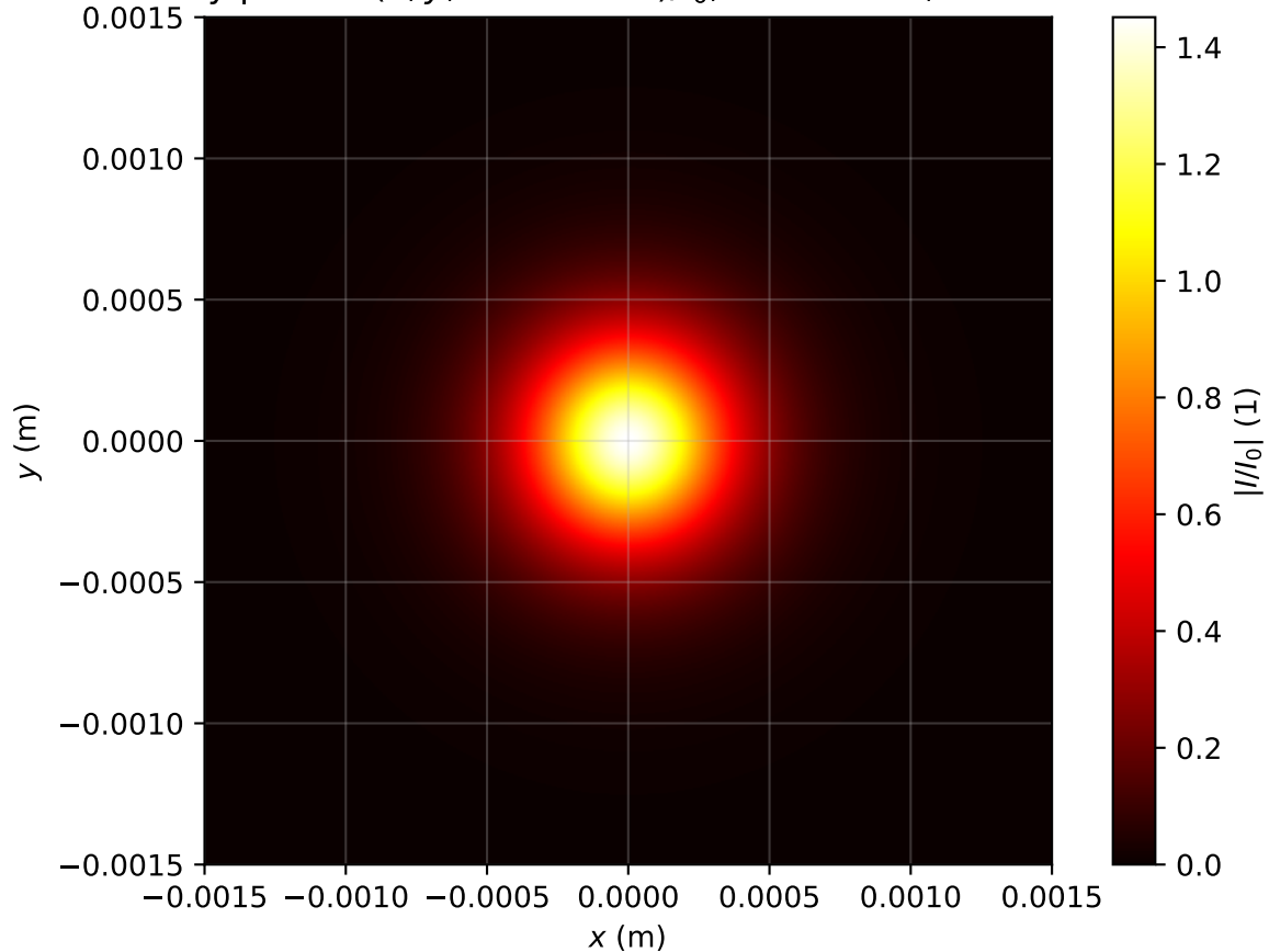
Intensity profile I(x, y, z = 3.742m)/I_0 , Pin=0.9Pcr, artificial time
